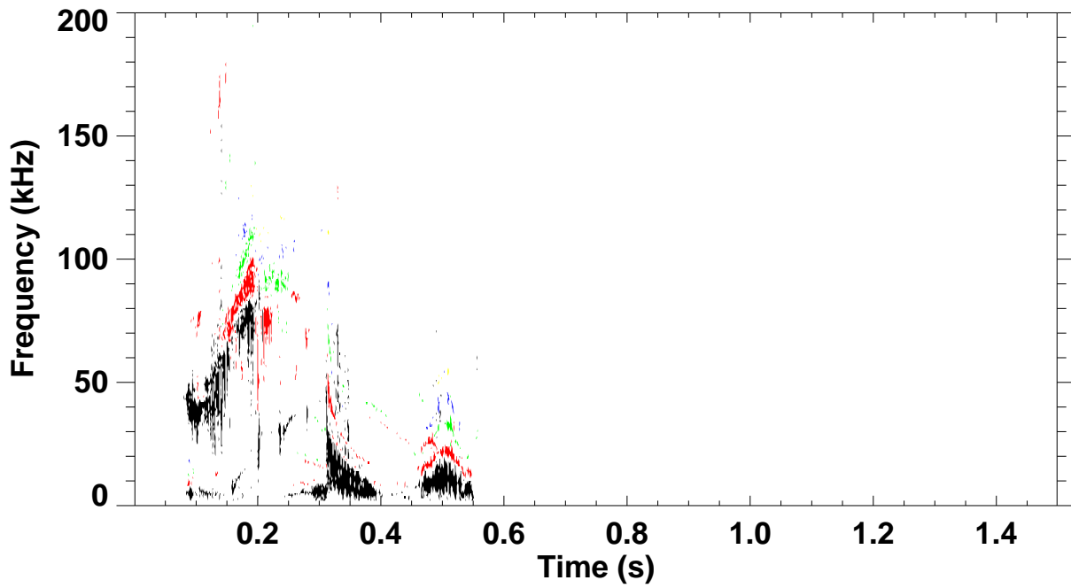
Shot 132198 \omega B(\omega) spectrum for toroidal mode number: 1 2 3 4 5
