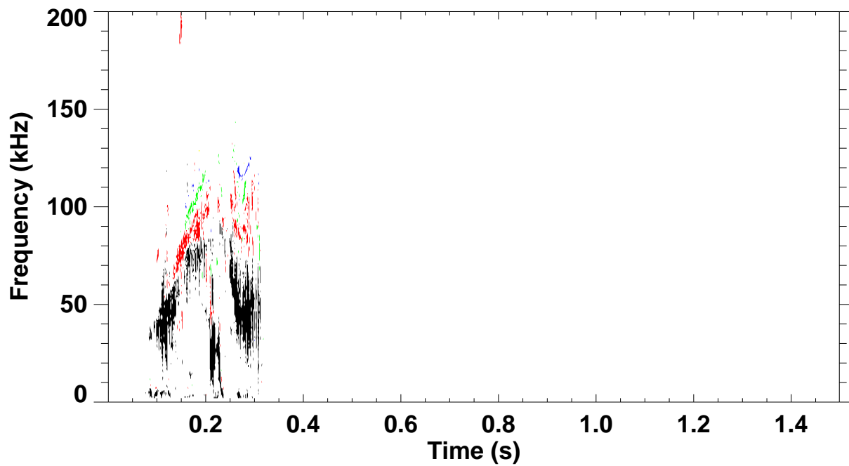
Shot 132201 \omega_B(\omega) spectrum for toroidal mode number: 1 2 3 4 5
