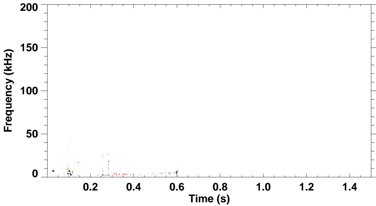
Shot 132488 \omega B(\omega) spectrum for toroidal mode number: 1 2 3 4 5
