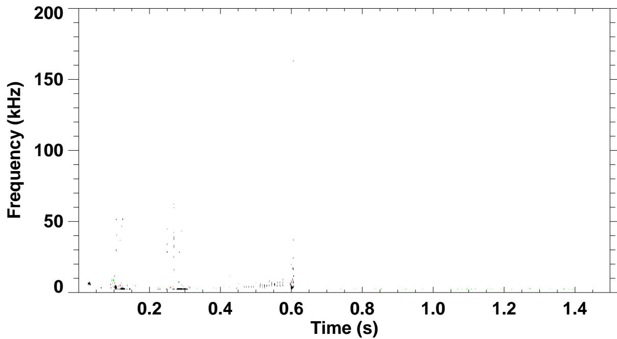
Shot 132505 \omega B(\omega) spectrum for toroidal mode number: 1 2 3 4 5
