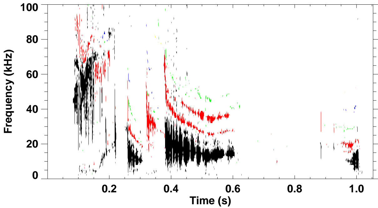
Shot 132566 \omega B(\omega) spectrum for toroidal mode number: 1 2 3 4 5
