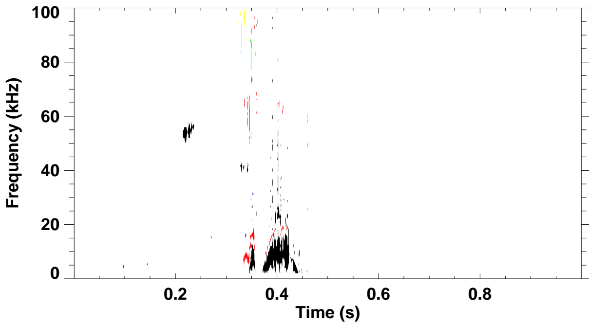
Shot 132691 \omega_B(\omega) spectrum for toroidal mode number: 1 2 3 4 5
