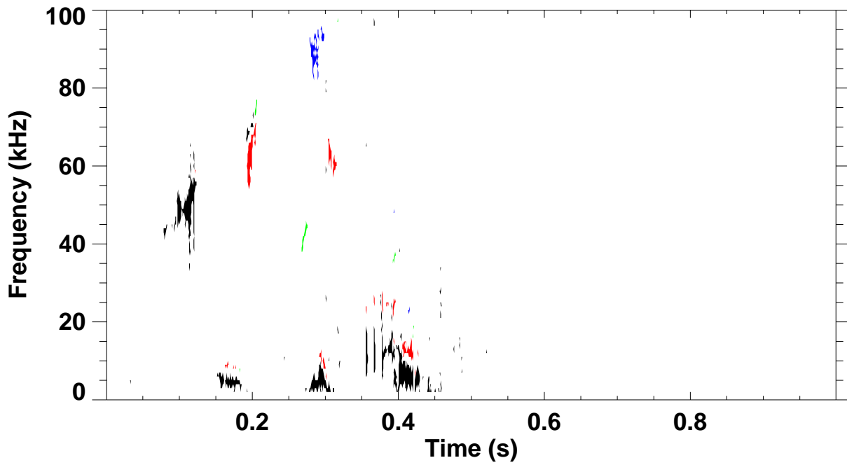
Shot 132710 \omega_B(\omega) spectrum for toroidal mode number: 1 2 3 4 5
