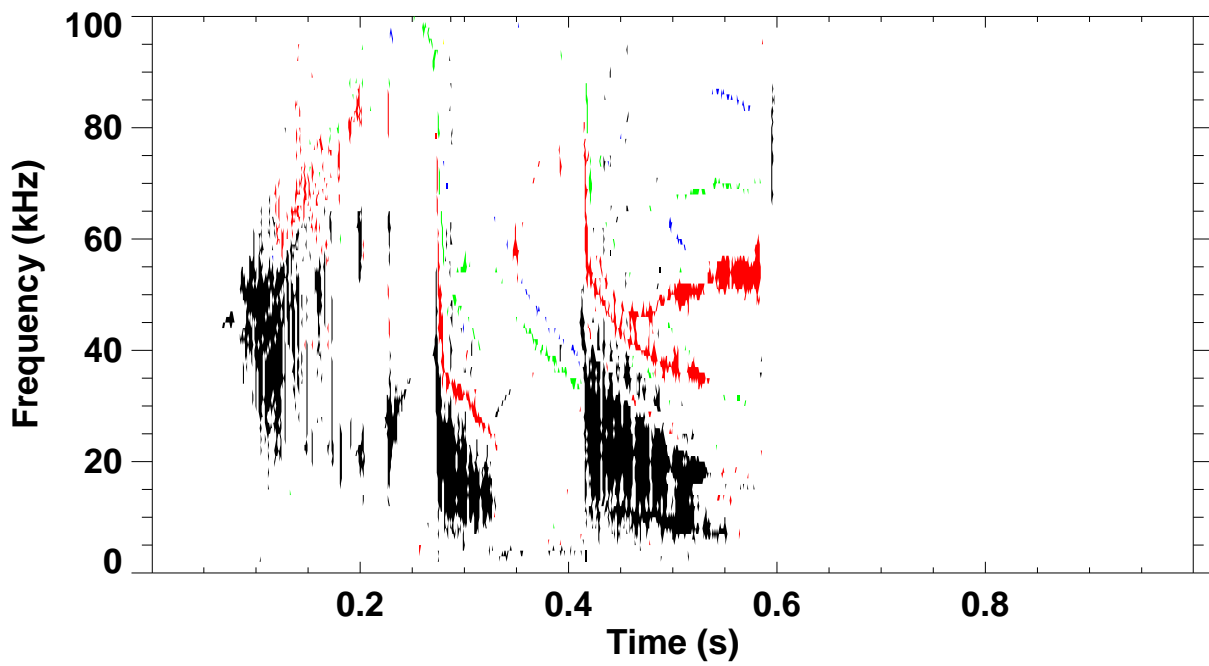
Shot 132731 \omega B(\omega) spectrum for toroidal mode number: 1 2 3 4 5
