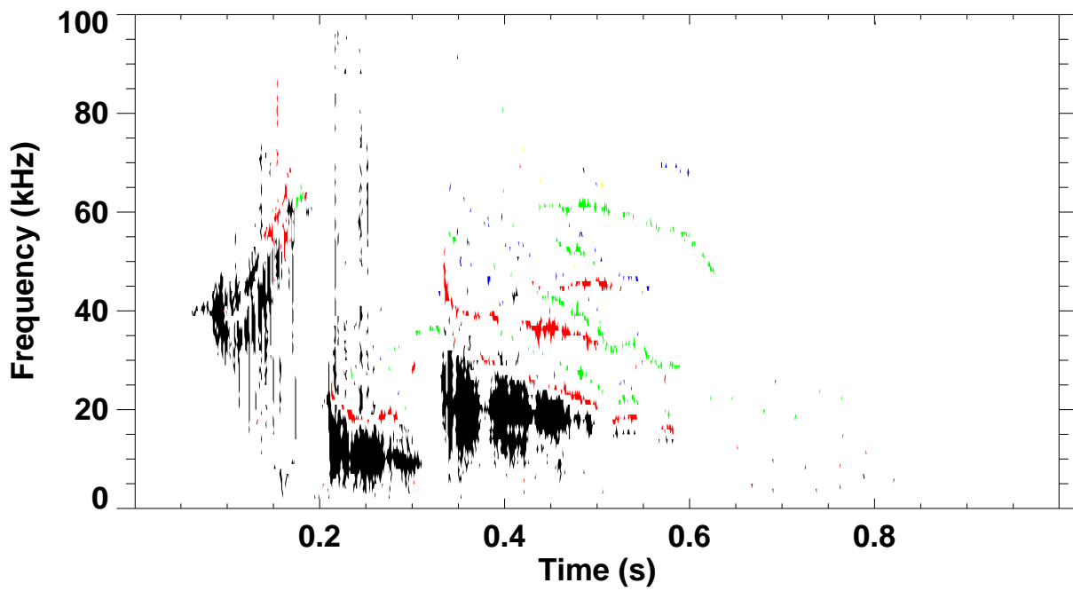
Shot 132802 \omega B(\omega) spectrum for toroidal mode number: 1 2 3 4 5
