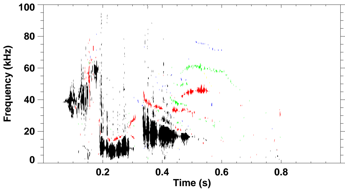
Shot 132803 \omega_B(\omega) spectrum for toroidal mode number: 1 2 3 4 5
