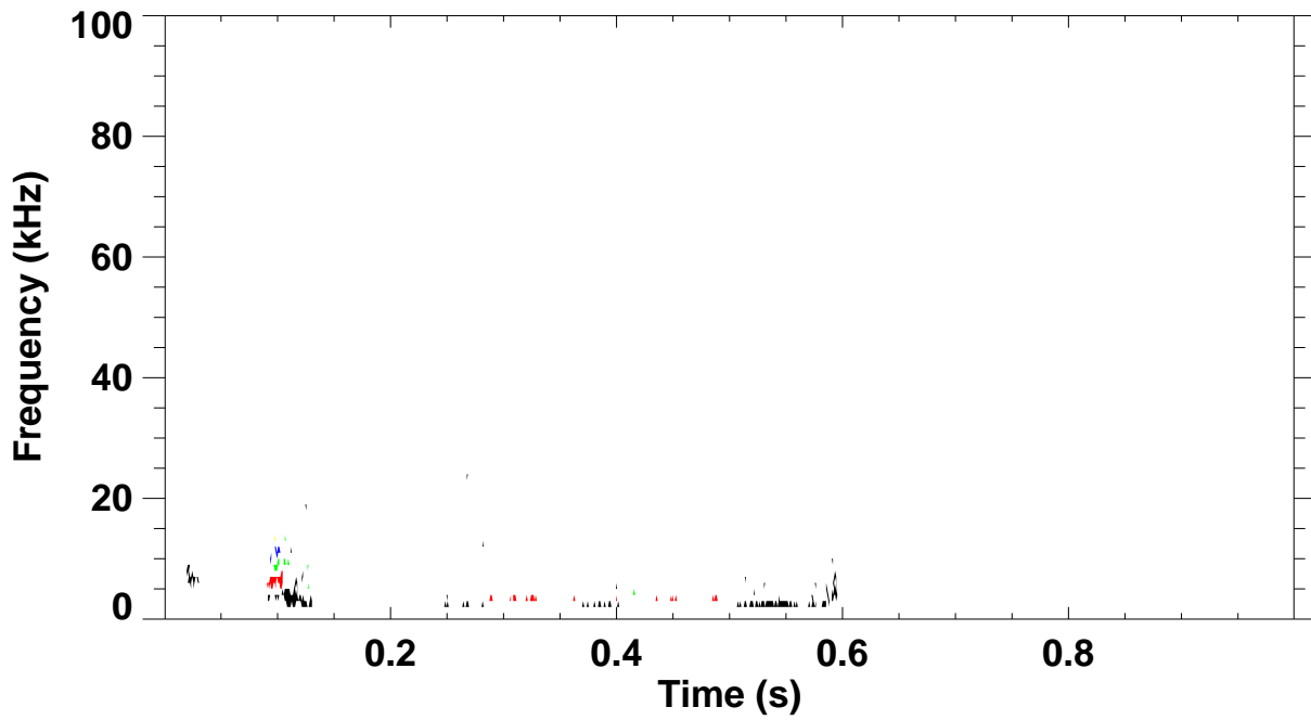
Shot 132978 \omega B(\omega) spectrum for toroidal mode number: 1 2 3 4 5
