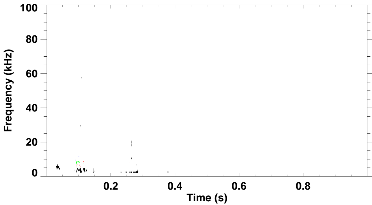
Shot 132987 \omega_B(\omega) spectrum for toroidal mode number: 1 2 3 4 5
