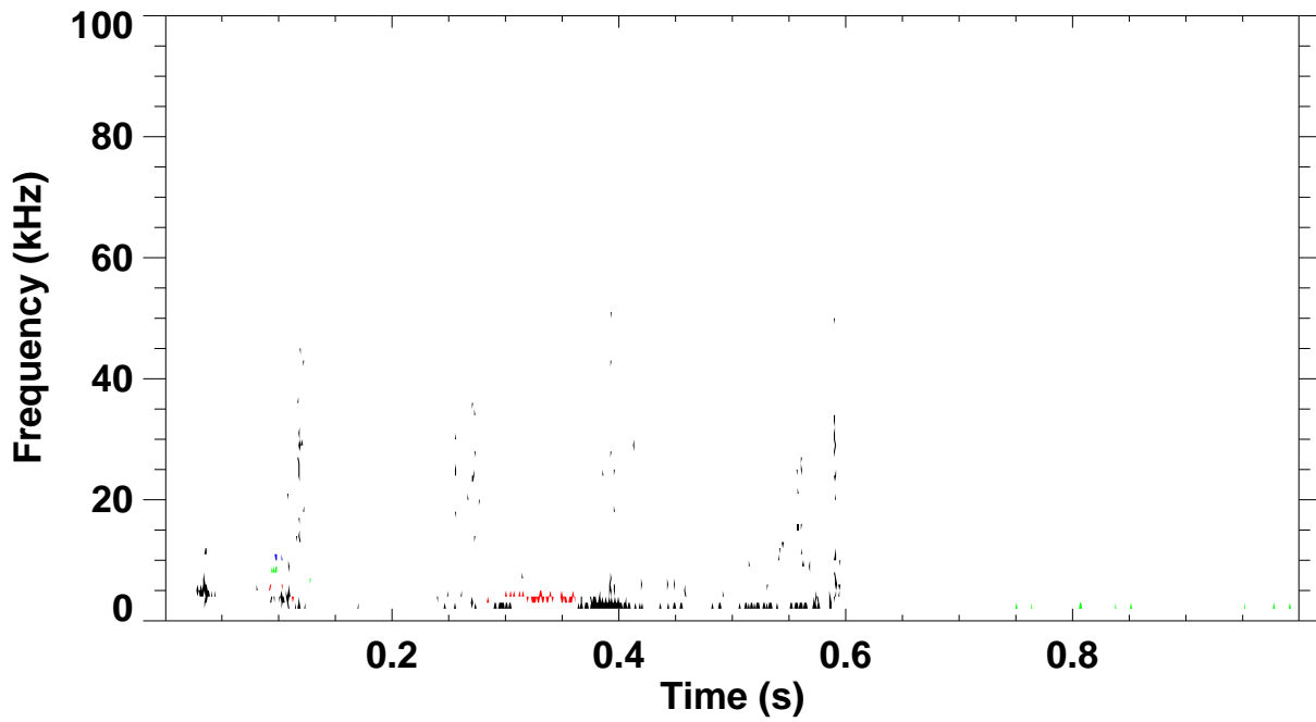
Shot 132991 \omega B(\omega) spectrum for toroidal mode number: 1 2 3 4 5
