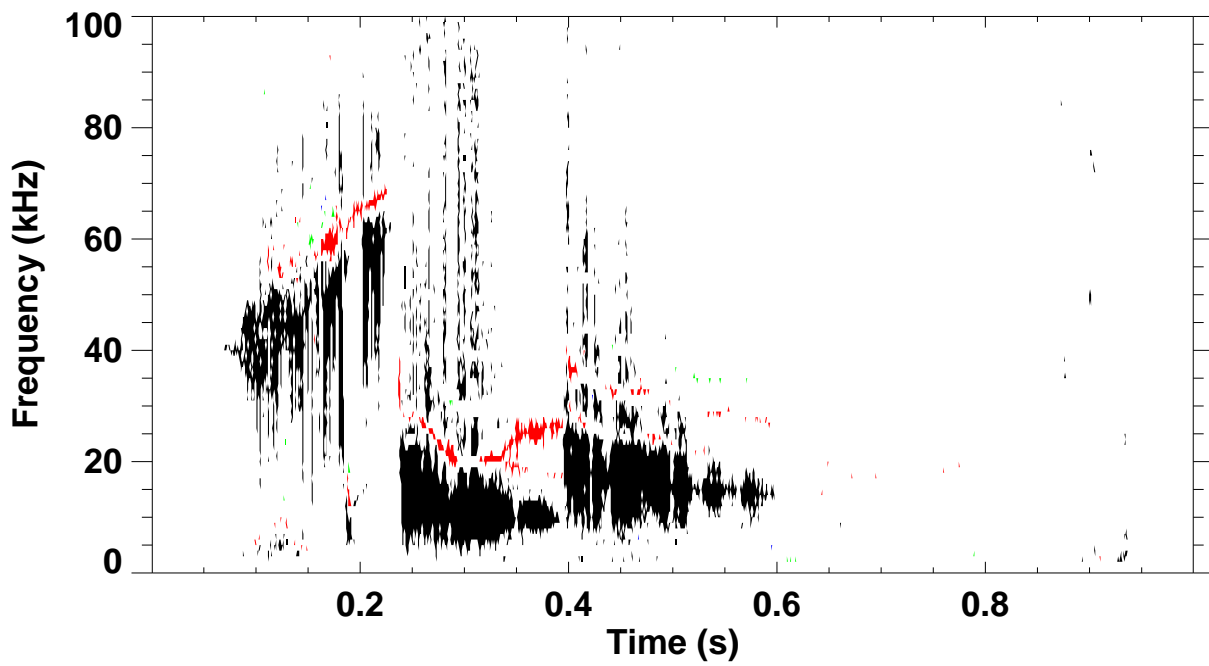
Shot 133236 \omega B(\omega) spectrum for toroidal mode number: 1 2 3 4 5
