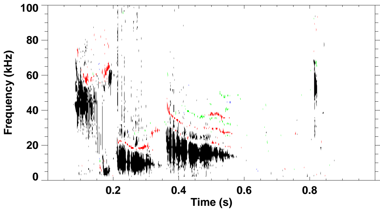
Shot 133357 \omega B(\omega) spectrum for toroidal mode number: 1 2 3 4 5
