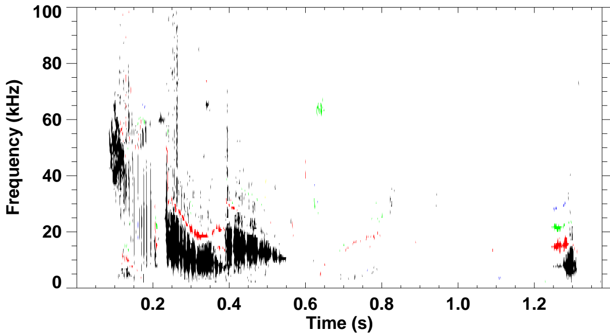
Shot 133750 \omega B(\omega) spectrum for toroidal mode number: 1 2 3 4 5
