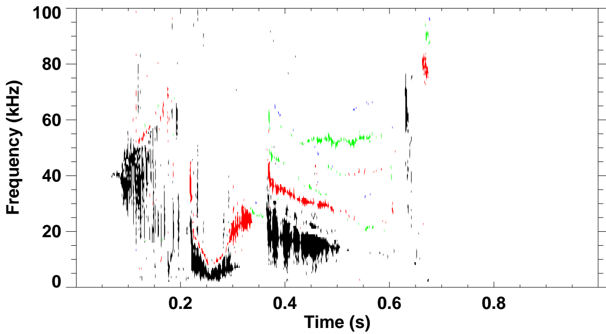
Shot 133921 \omega B(\omega) spectrum for toroidal mode number: 1 2 3 4 5
