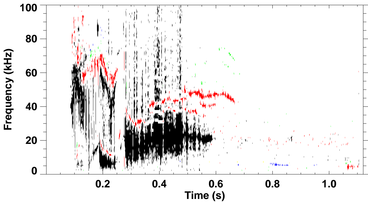
Shot 133975 \omega B(\omega) spectrum for toroidal mode number: 1 2 3 4 5
