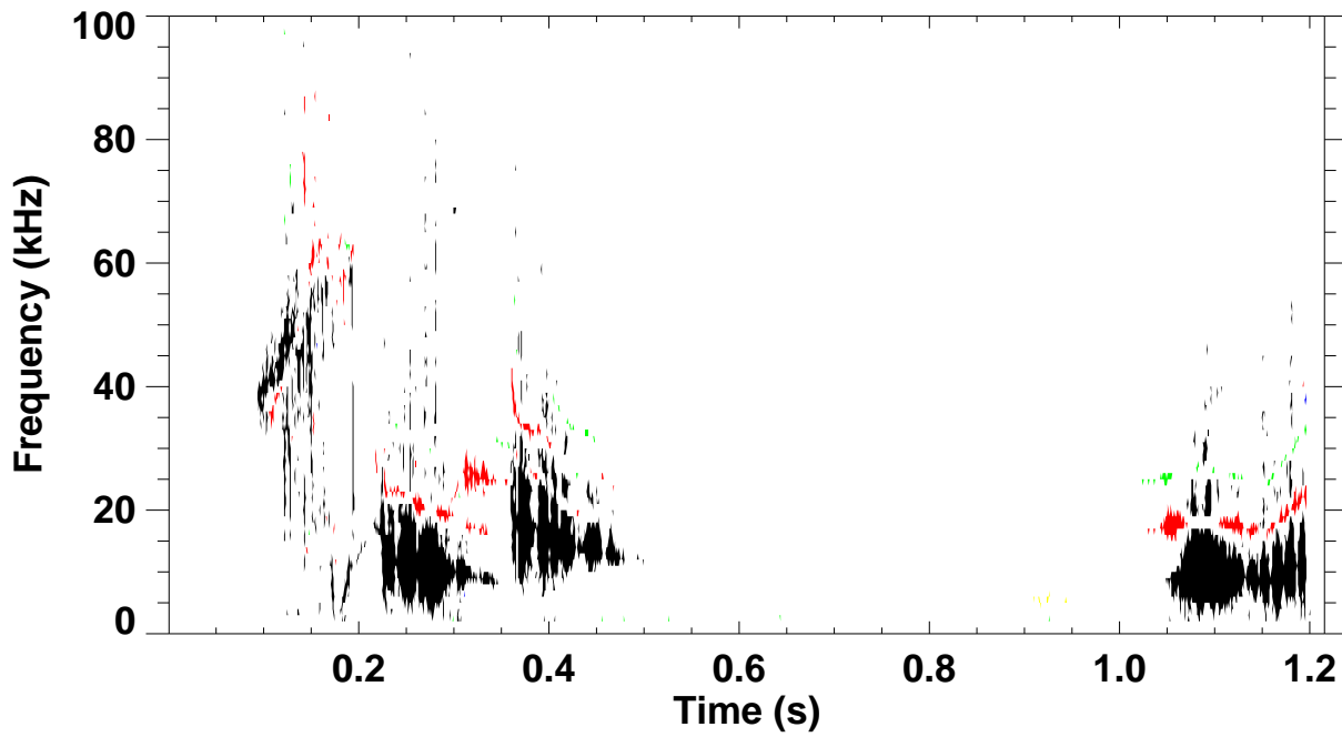
Shot 134130 \omega B(\omega) spectrum for toroidal mode number: 1 2 3 4 5
