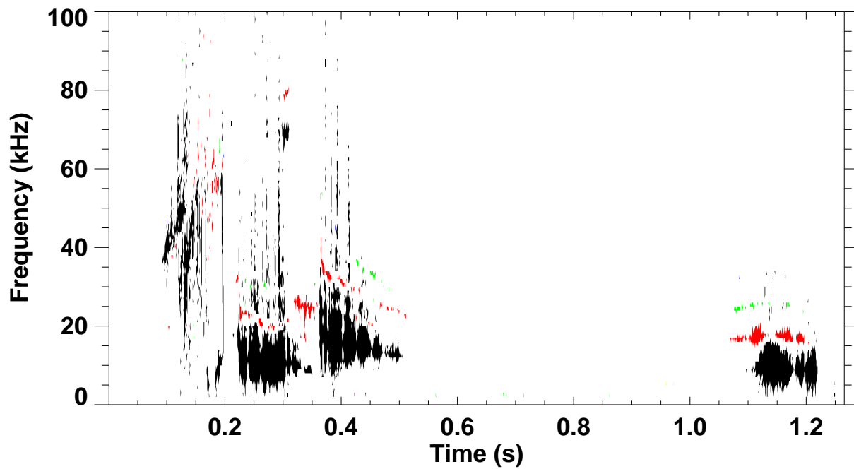
Shot 134136 \omega B(\omega) spectrum for toroidal mode number: 1 2 3 4 5
