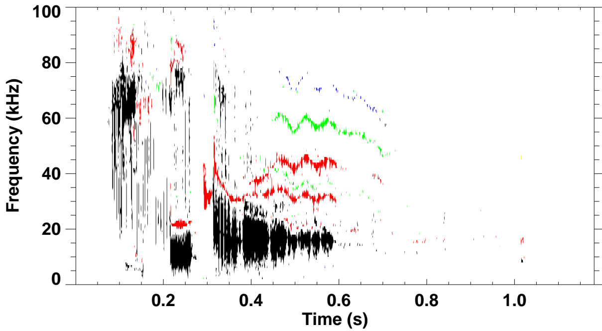
Shot 134331 \omega B(\omega) spectrum for toroidal mode number: 1 2 3 4 5
