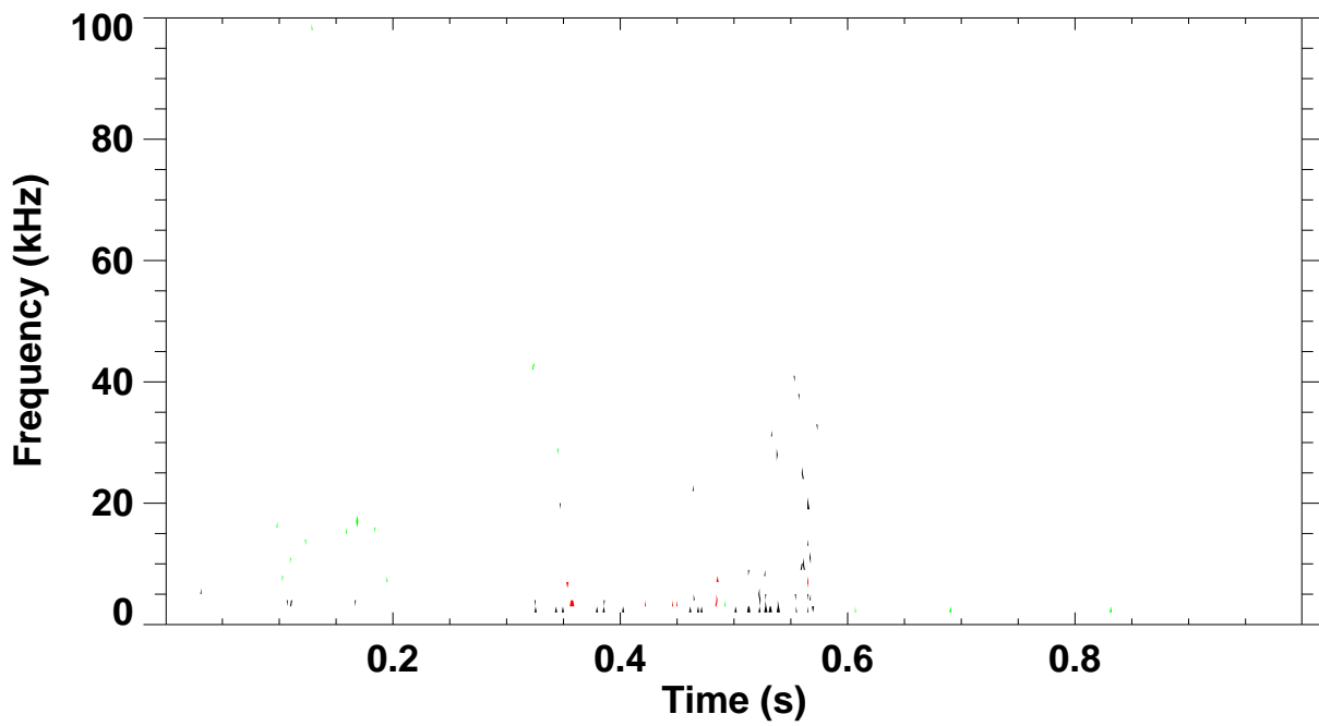
Shot 134696 \omega B(\omega) spectrum for toroidal mode number: 1 2 3 4 5
