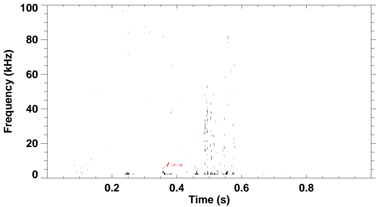
Shot 134703 \omega_B(\omega) spectrum for toroidal mode number: 1 2 3 4 5
