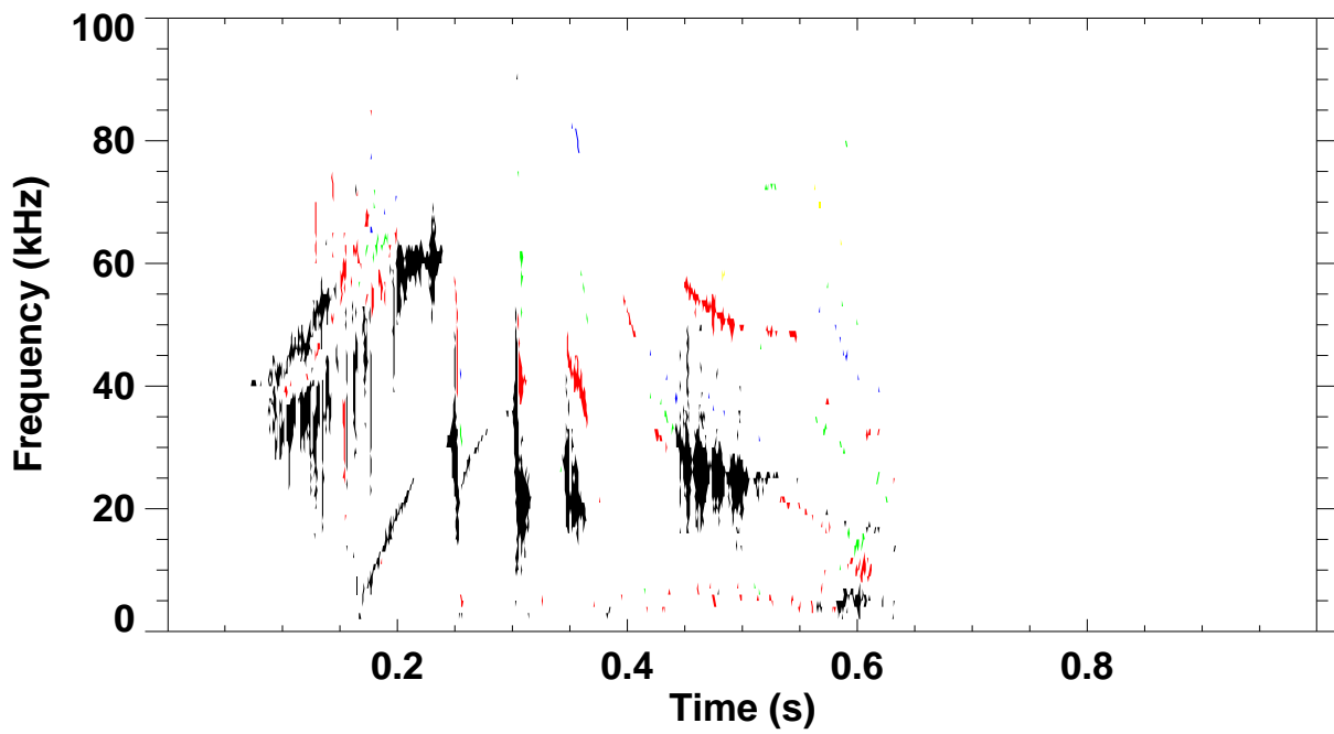
Shot 134740 \omega B(\omega) spectrum for toroidal mode number: 1 2 3 4 5
