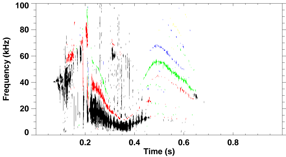
Shot 134768 \omega B(\omega) spectrum for toroidal mode number: 1 2 3 4 5
