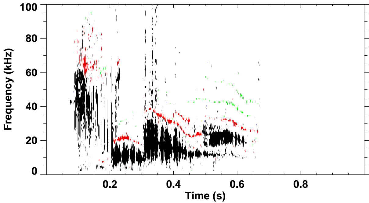
Shot 134786 \omega B(\omega) spectrum for toroidal mode number: 1 2 3 4 5
