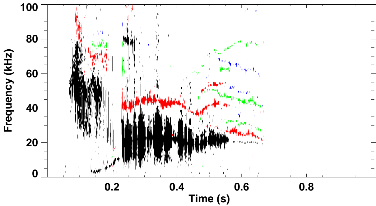
Shot 134797 \omega B(\omega) spectrum for toroidal mode number: 1 2 3 4 5
