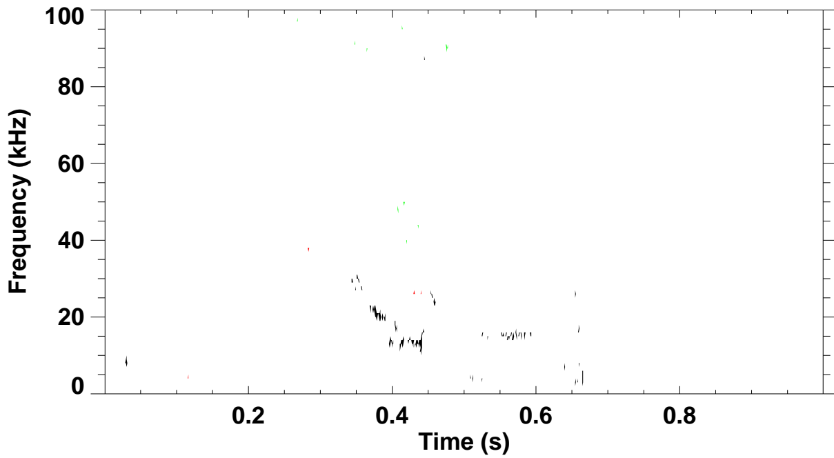
Shot 135285 \omega_B(\omega) spectrum for toroidal mode number: 1 2 3 4 5
