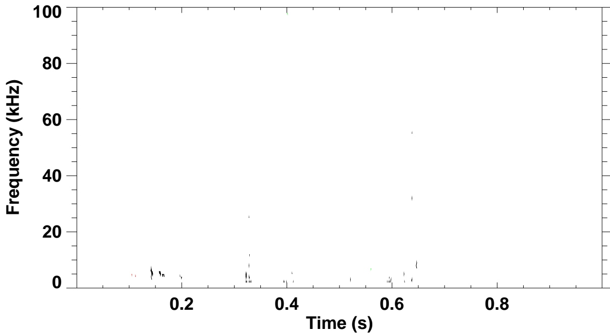
Shot 135291 \omega_B(\omega) spectrum for toroidal mode number: 1 2 3 4 5
