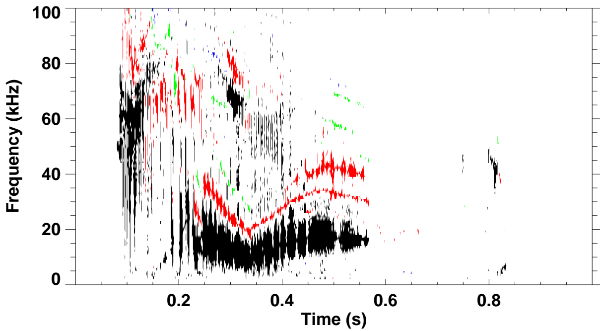
Shot 135780 \omega B(\omega) spectrum for toroidal mode number: 1 2 3 4 5
