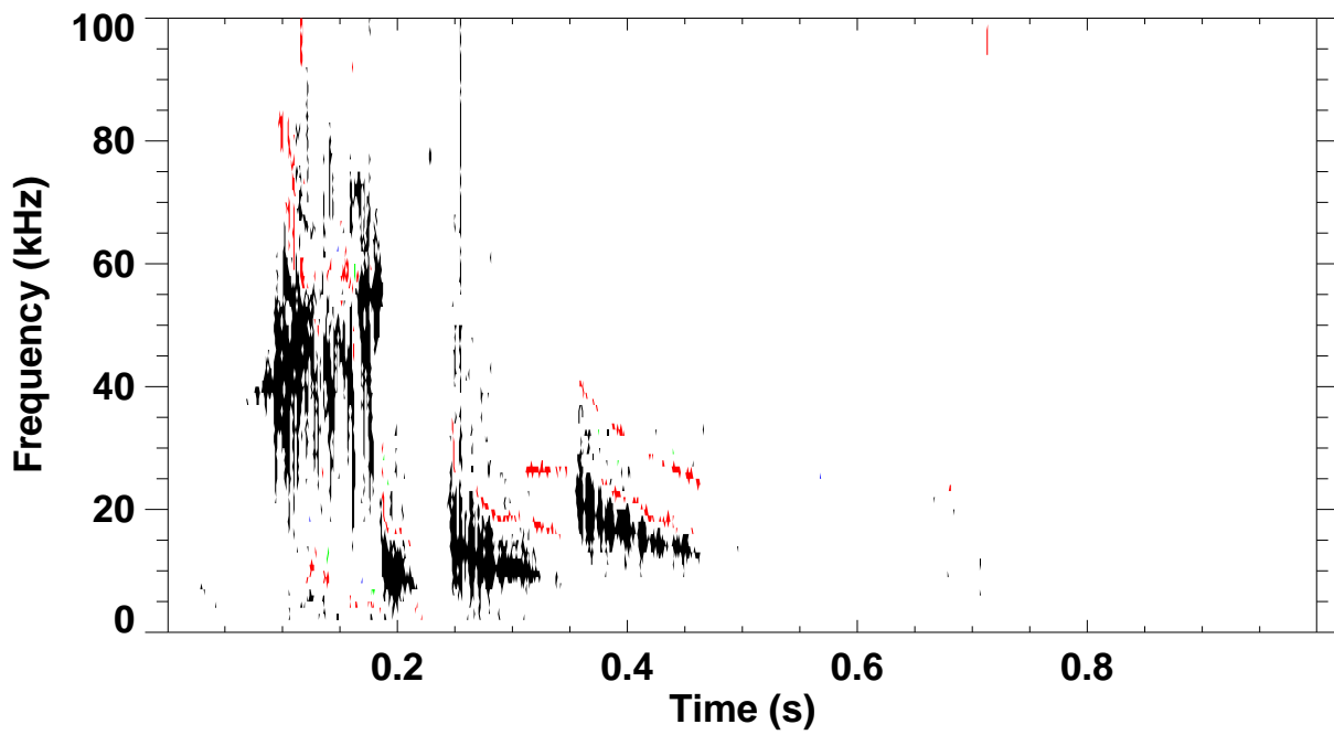
Shot 135846 \omega B(\omega) spectrum for toroidal mode number: 1 2 3 4 5
