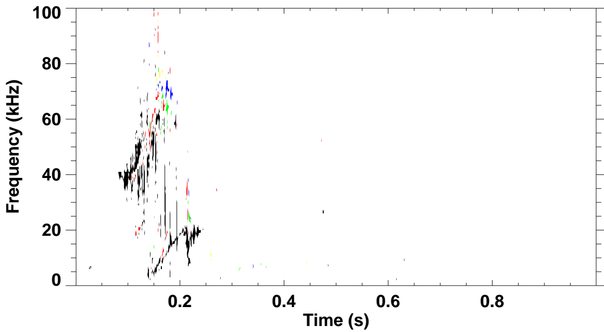
Shot 135951 \omega B(\omega) spectrum for toroidal mode number: 1 2 3 4 5
