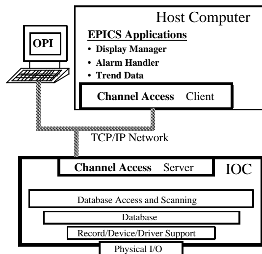
Fig. 1 Basic EPICS Architecture
