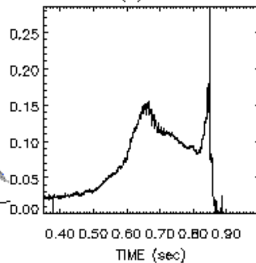
Est. Z_{\text{eff}}(0) from metals
