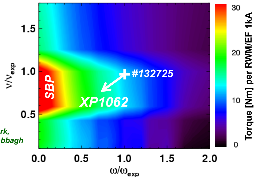
NSTX NTV n=3 braking vs. (\nu, \omega_\phi) by IPEC+NTV
