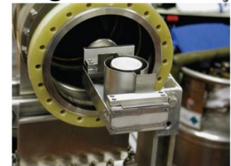
Y 2 O 3 crucible, Ta heater ➤ Tested to 700 °C
