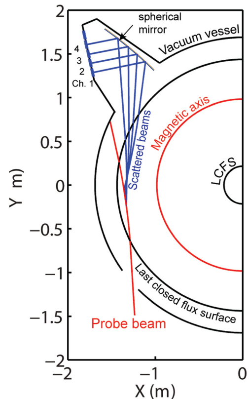
FIG. 1. (a) Experimental configuration of high- k scattering experiment for shot 141767 (view from the top). Probe beam is launched nearly on the mid-plane. Gaussian beam propagation is calculated using a ray-tracing code.
