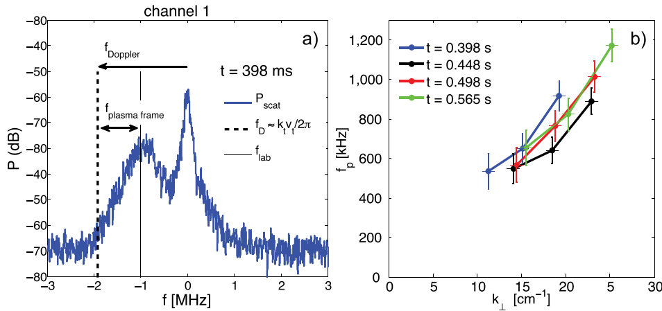
FIG. 6. (a) Scattered power from channel 1 of high- k scattering diagnostic, at time t = 398 ms. Fluctuation frequencies are Doppler shifted by f_D \approx k_r v_i / 2\pi . The plasma frame frequency of fluctuations f_p is obtained by f_p = f_{lab} - f_D . (b) Dispersion relation obtained experimentally from measured electron density fluctuations.
