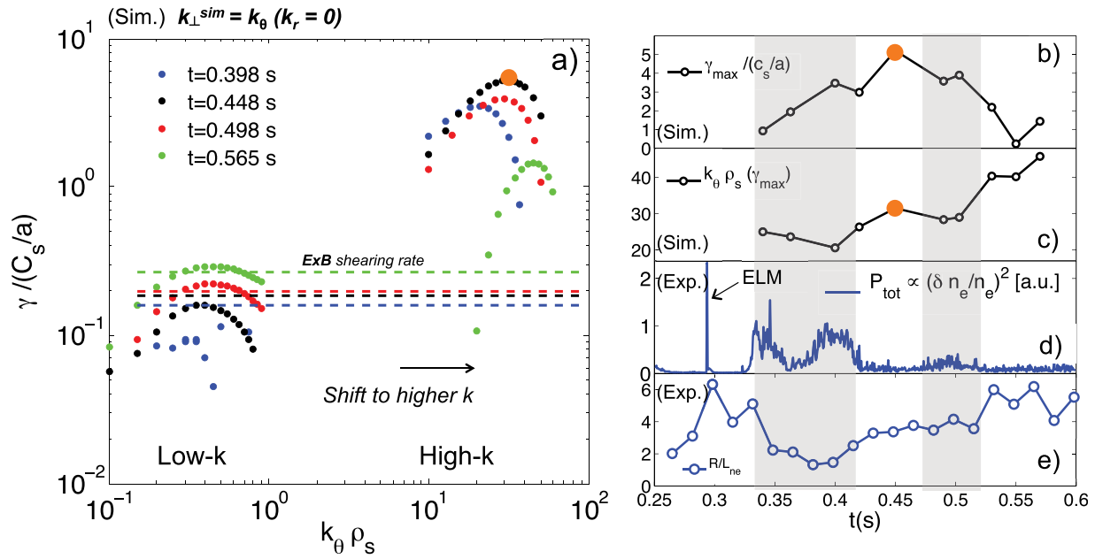
FIG. 14. (a) Linear growth rates computed with GS2 for low-k ( 0.1 \leq k_\theta \rho_s \leq 1 ) and high-k wavenumbers ( 10 \leq k_\theta \rho_s \leq 60 ). Notice the linearly unstable high-k wavenumbers are shifting to even higher wavenumbers as time progresses. Horizontal lines correspond to E \times B shearing rate from TRANSP calculations (Waltz-Miller definition 24 ). (b) Maximum linear growth rate computed with GS2. (c) Wavenumber corresponding to the maximum growth rate computed with GS2. (d) Total scattered power (integrated in frequency) from channel 1 of the high-k scattering diagnostic. (e) Normalized electron density gradient R_0/L_{n_e} computed at the scattering location. Notice the similarity between Figures 14(c) and 14(e).
