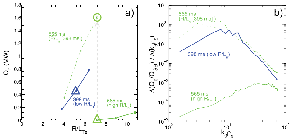
FIG. 12. (a) Predicted electron heat flux by GYRO as a function of R_0/L_{Te} for the high R_0/L_{ne} case (green) and low R_0/L_{ne} case (blue). Experimental cases are shown by blue and green triangles. The green dashed line shows the predicted heat flux at t = 565 ms, but using the density gradient value from t = 398 ms. The green circle is calculated by only varying the density gradient from t = 565 ms (green triangle) to the value at t = 398 ms (low R_0/L_{ne} ). Note the consequent impact on Q_e . (b) Fractional electron heat flux spectrum corresponding to the experimental base cases (green and blue triangles), and at t = 565 ms using the R_0/L_{ne} value from t = 398 ms (corresponding to green circle in (a)).
