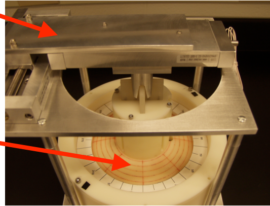
18-40 GHz EBW Antenna
