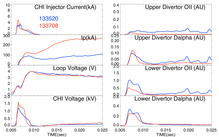
Figure 4. The CHI discharge indicated in blue was taken early in the CHI campaign, while the one in red was benefited from discharge cleaning Li evaporation. Both CHI discharges used 10 mF at 1.7 kV.
