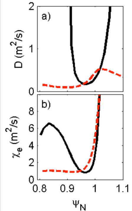
Fig. 1 – Comparison of computed a) particle and b) electron thermal diffusivity for pre-li (solid black - #129015) and post-li (dashed red - #129038) discharges.
