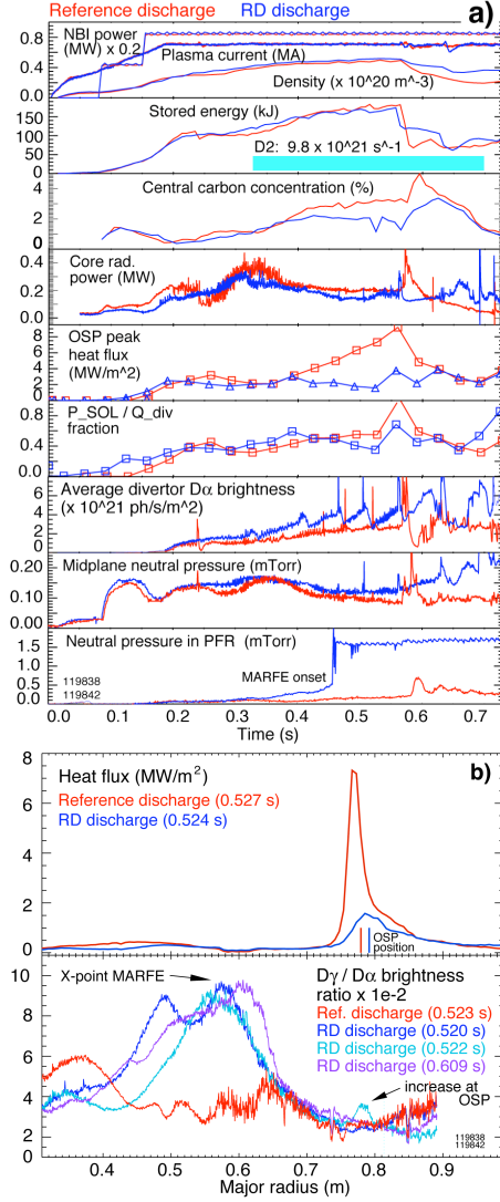
Figure 2: Signal time histories (a) and divertor profiles (b) of a reference and a RD discharges
