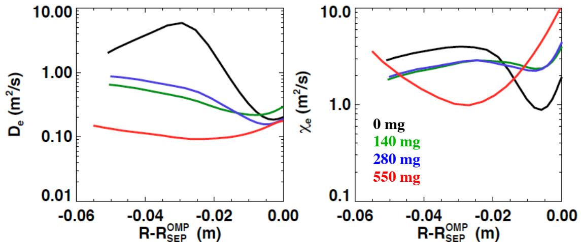
Figure 6: (a) effective electron particle diffusivity D_e and (b) electron thermal conductivity \chi_e vs. distance from the separatrix at the outer midplane. The lithium evaporation dose is indicated.
