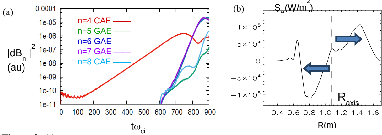
Figure 2. (a) Time evolution of amplitudes of different toroidal harmonics from nonlinear simulations for NSTX shot 141398; (b) Radial component of Poynting vector \mathbf{S} = \langle \mathbf{E} \times \mathbf{B} \rangle at the midplane at t=750 .
