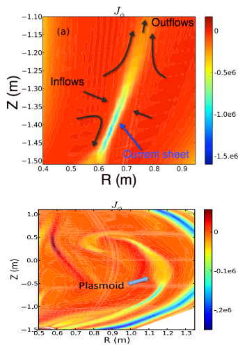
Fig1: Top: Elongated current sheet formation during forced S-P reconnection. Bottom: Current sheet breaks up due to spontaneous reconnection at high S .
