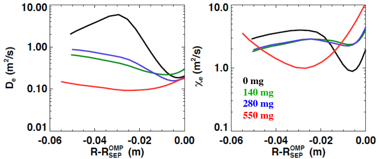
Figure 2: (a) effective electron particle diffusivity D_e and (b) electron thermal conductivity \chi_e vs. distance from the separatrix at the outer midplane. The lithium evaporation dose is indicated.
